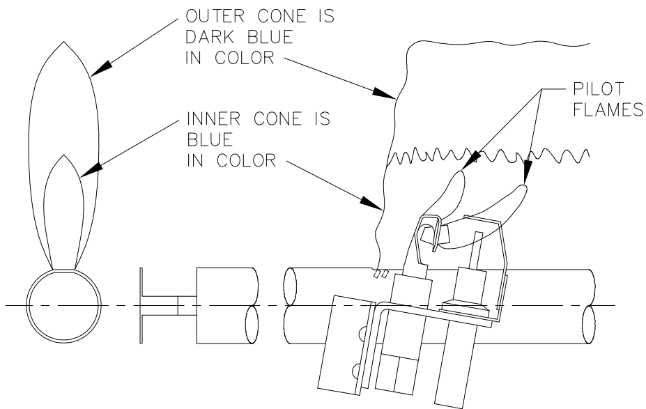
Figure 5: Intermittent Ignition Pilot Configuration and Flames
