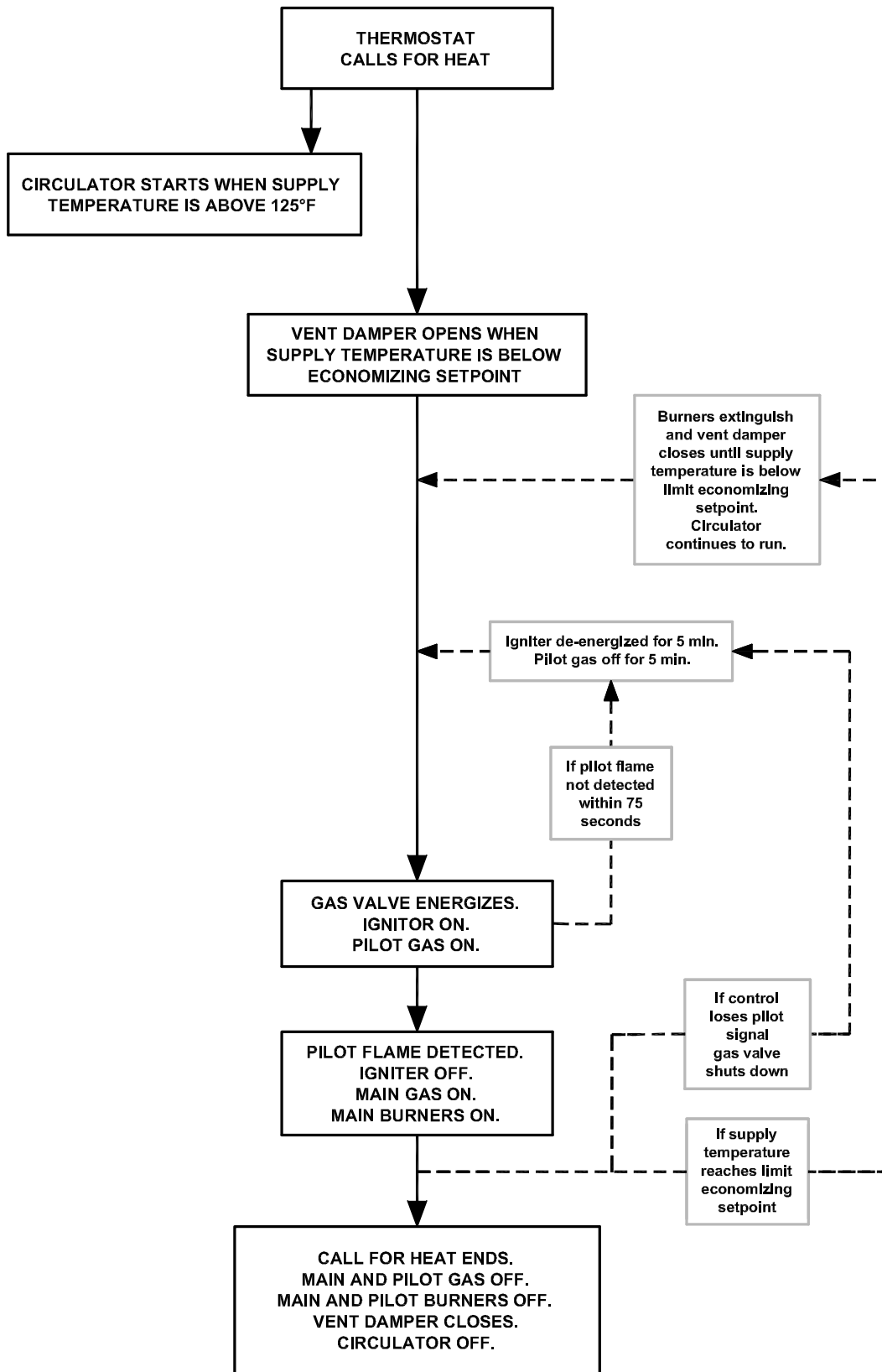
Figure 4: Intermittent Ignition Sequence of Operation
